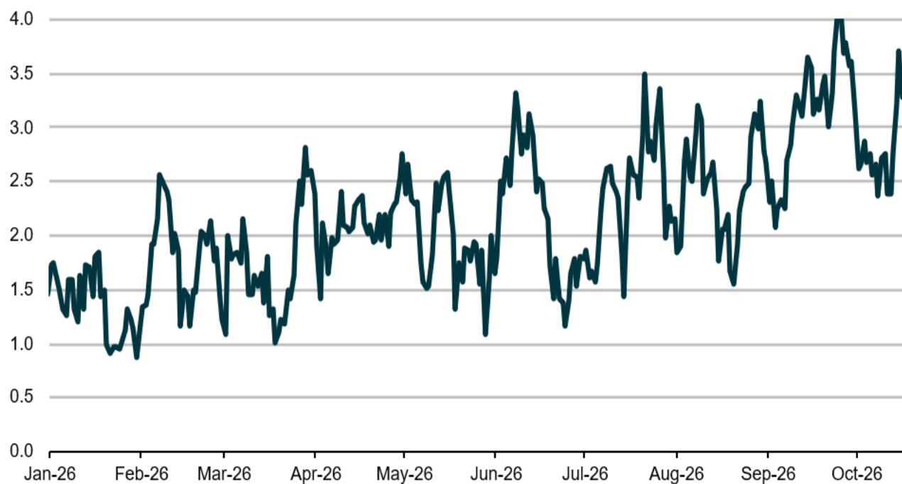
Fujairah - Total oil (crude + products) export (7-dma, mb/d)
