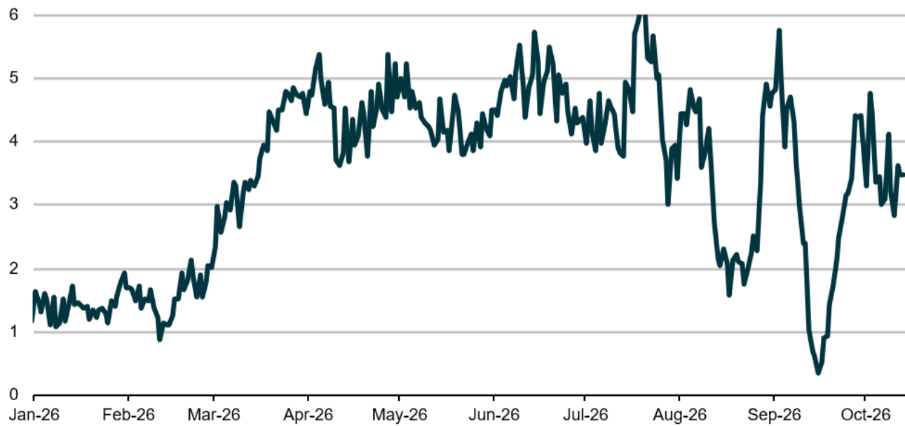
Yanbu - total oil (crude + products) export (7-dma, mb/d)
